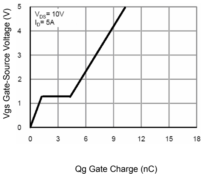
Figure 11 Gate Charge
