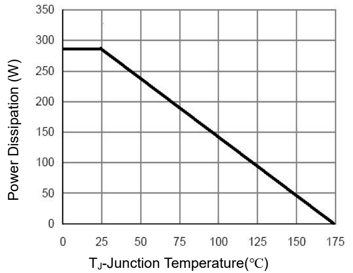
Figure 9 Power De-rating
